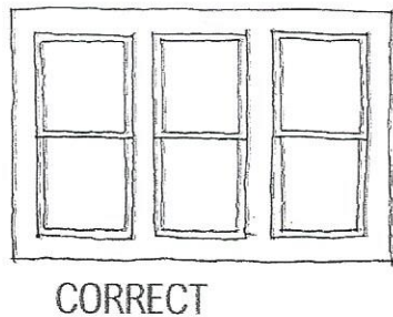
Multiple windows separated by full trim boards
