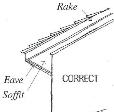
Sloped Soffit & Rake
